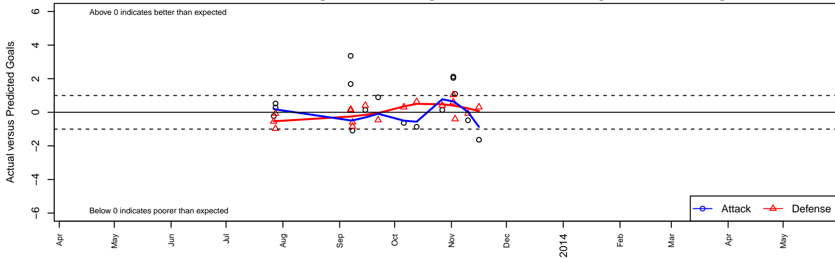
Cobra Dortmund B99 Dots are actual minus expected GF (blue circles) and GA (red triangles). Blue line is smoothed change in attack strength. Red is smoothed change in defense strength.
